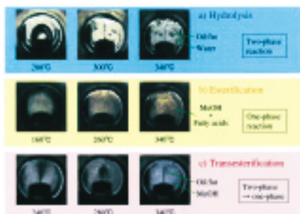
Fig.4 In-situ observations for the oil/fat reactions through a sapphire glass
